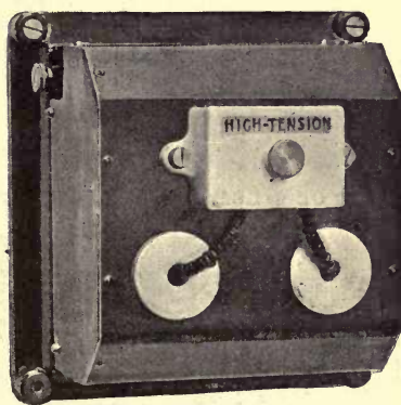
Fig. 138.—High-pressure Transformer
